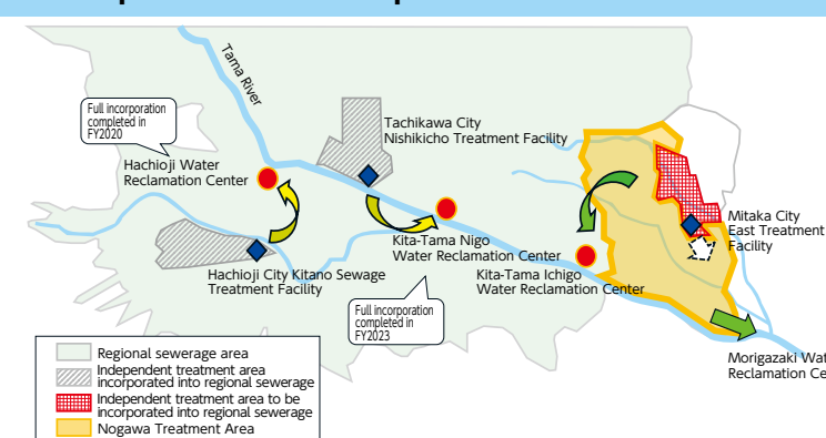
Construct of wastewater treatment facilities for independent treatment area incorporation (Hachioji Water Reclamation Center)
